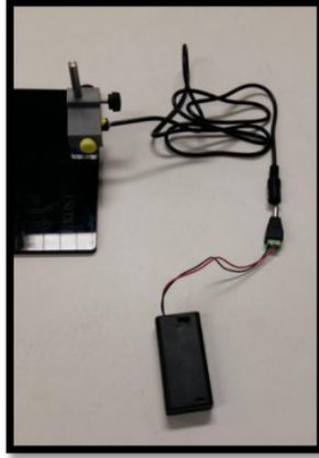
Figure 11: Laser diode connected to the battery pack.
