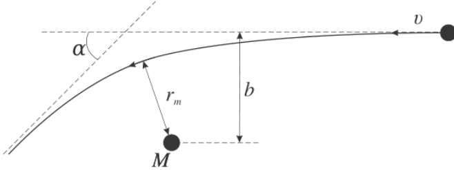
Fig. 1: The deflection of a star by the SBH with mass M . The impact parameter is b , the minimal distance between the star and the SBH is r_m .
