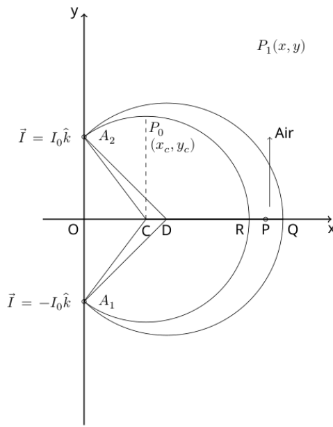
Figure 2: The arrangement for the inhomogeneous magnetic field
