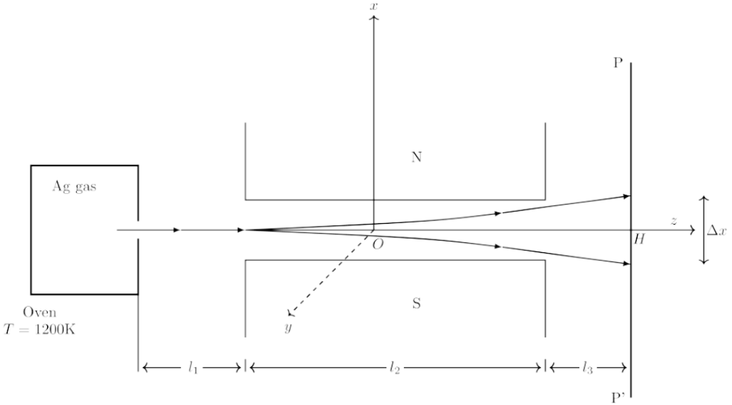
Figure 1: Schematic diagram of the Stern-Gerlach setup.
