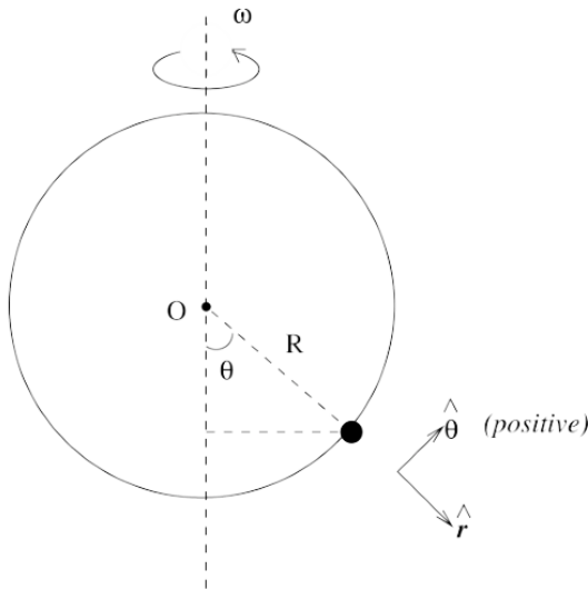
Fig. 1: The bead on a rotating ring.
