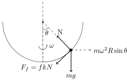
Fig. 2: The free body diagram.
