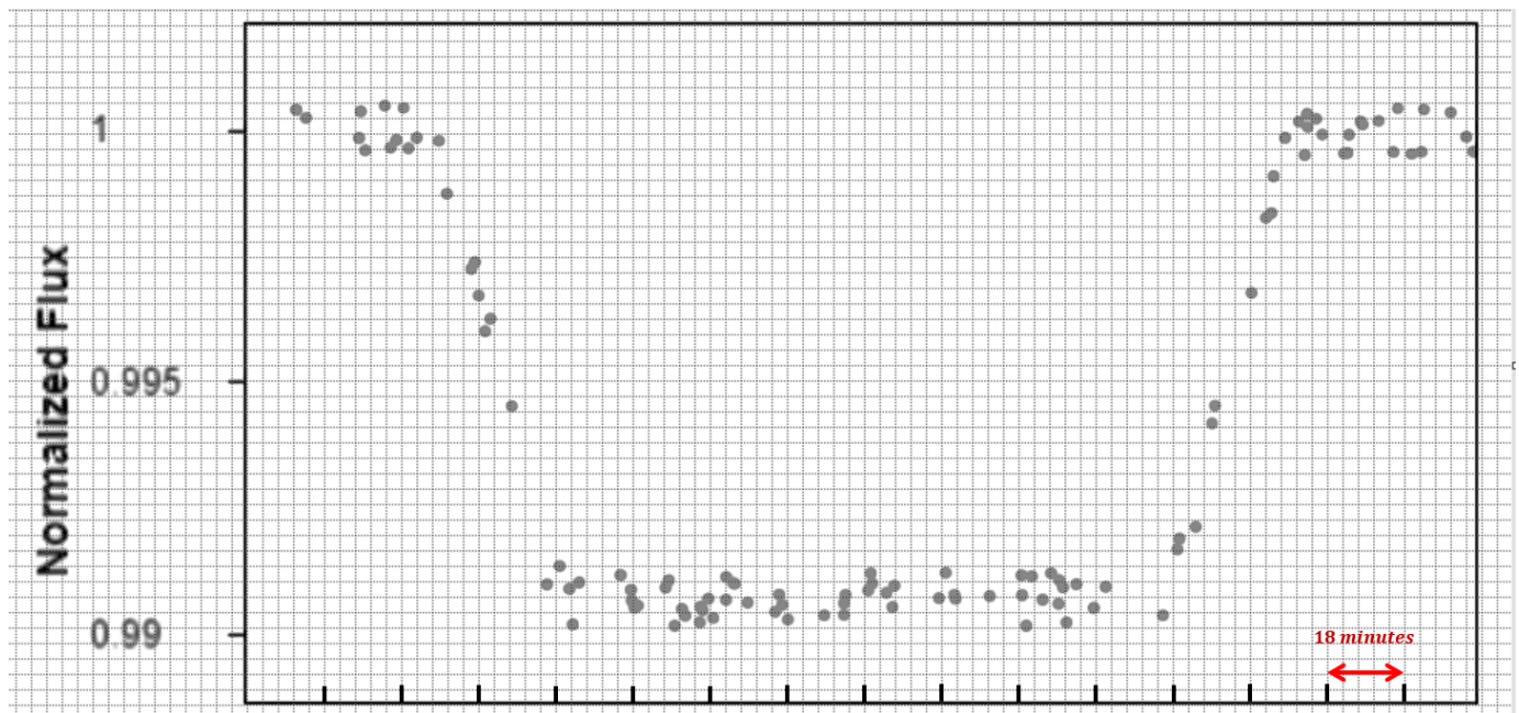
Figure 5: Normalized light curve: X-axis is time ( Every 5 grid lines are equal to 18 minutes! )
