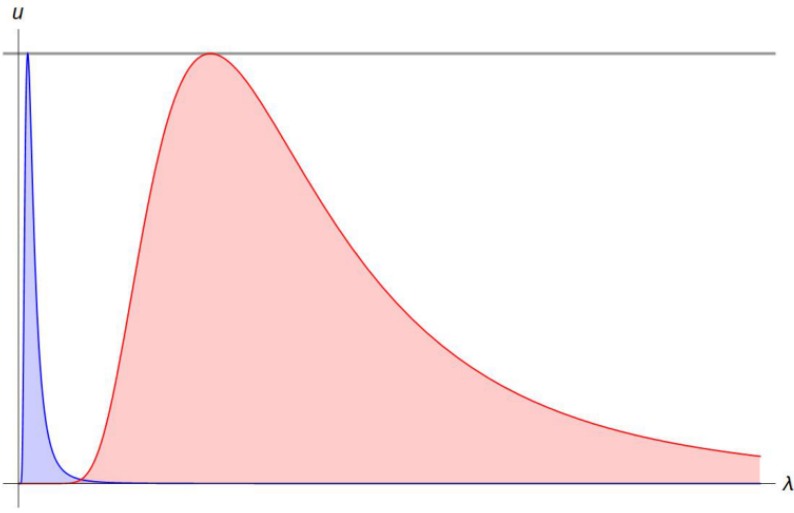
Figure 1 - The plot of u(\lambda, T_E) (red) and \gamma \tilde{u}_S(\lambda) (blue) versus \lambda
