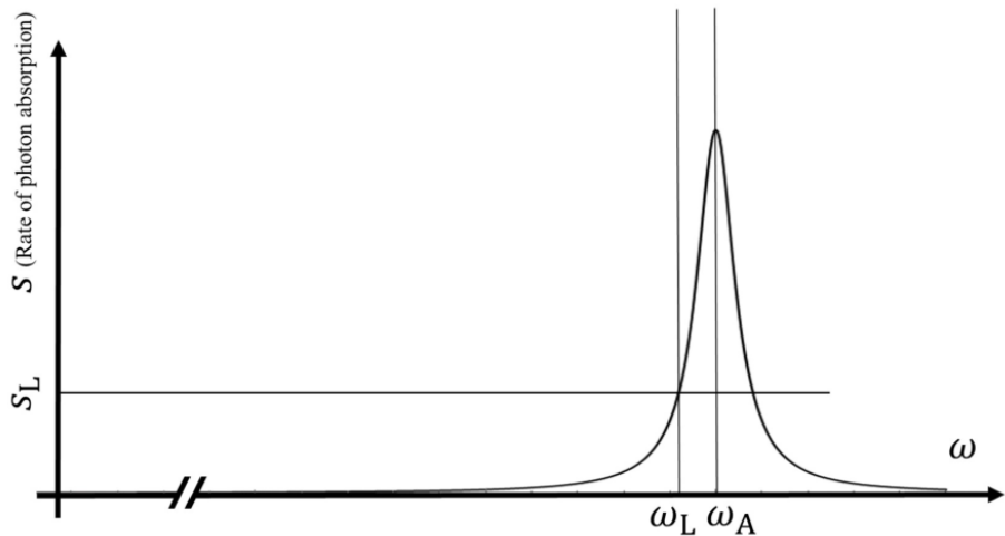
Figure 3 - The rate of photon absorption as a function of the frequency for a particular trap: the frequency corresponding to the energy difference between the two atomic levels is indicated by \omega_A and the slightly smaller frequency of the laser is indicated by \omega_L .
