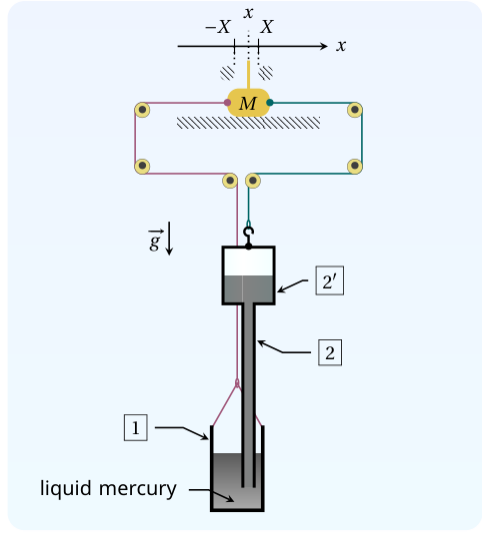
Fig. 6. Sketch of the system modeling the timepiece
