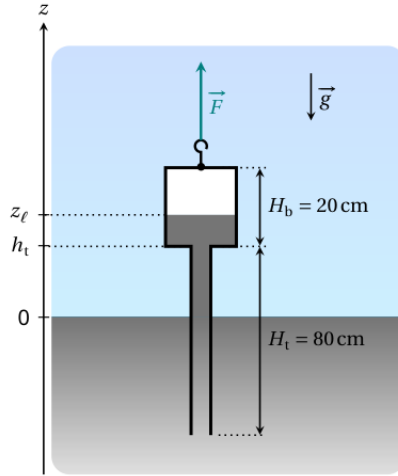
Fig. 3. Sketch of the two-part barometric tube
