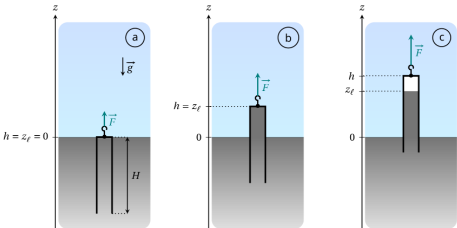
Fig. 2. Sketch of the tube in different configurations
