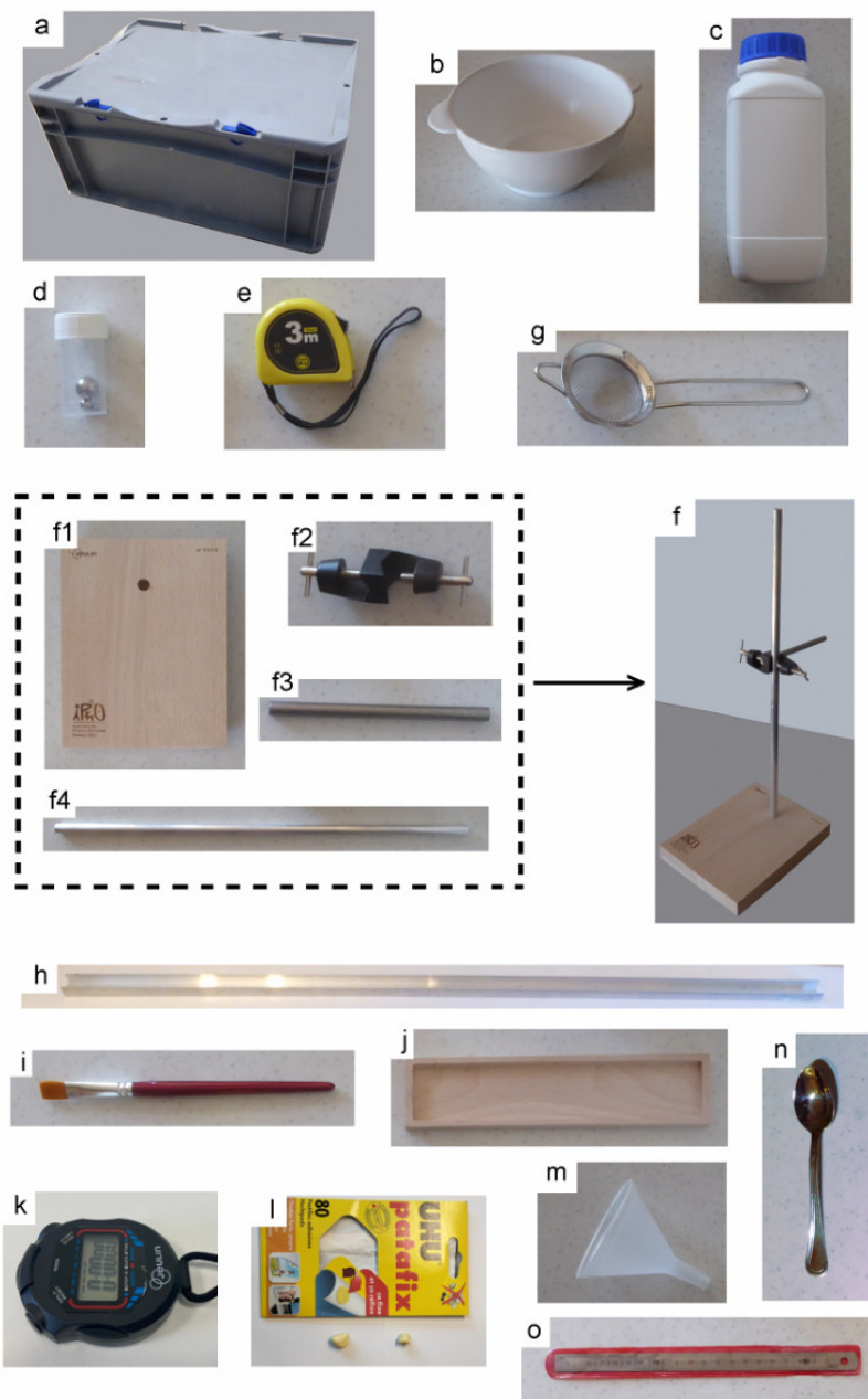
Fig. 2. Photographs of all equipment.
